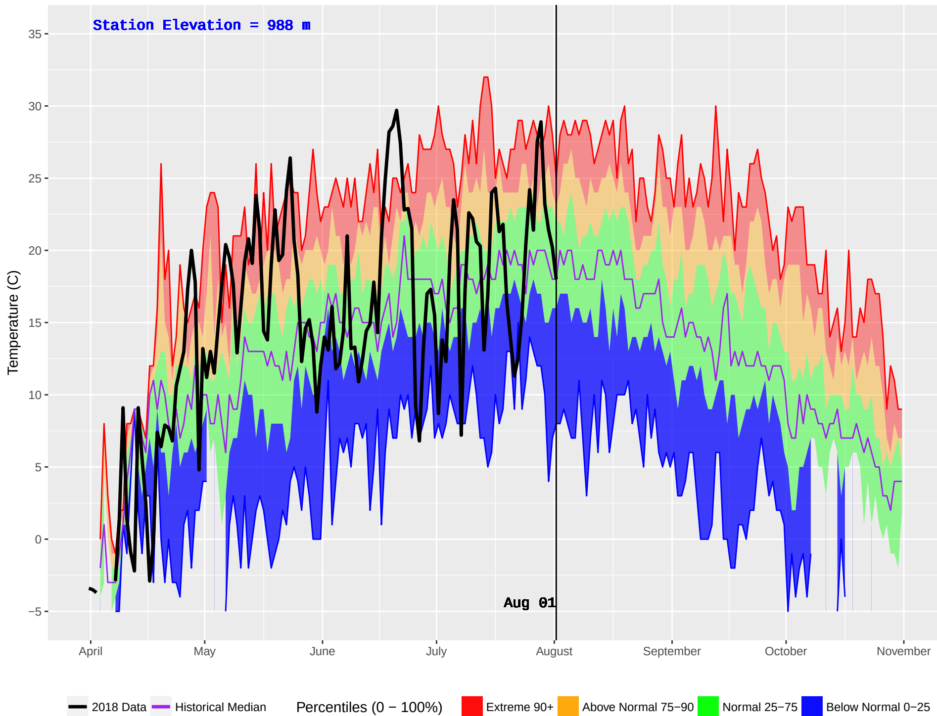
NOEL (437) : Historical (1993–2016) and Current (2018) Daily Temperature
