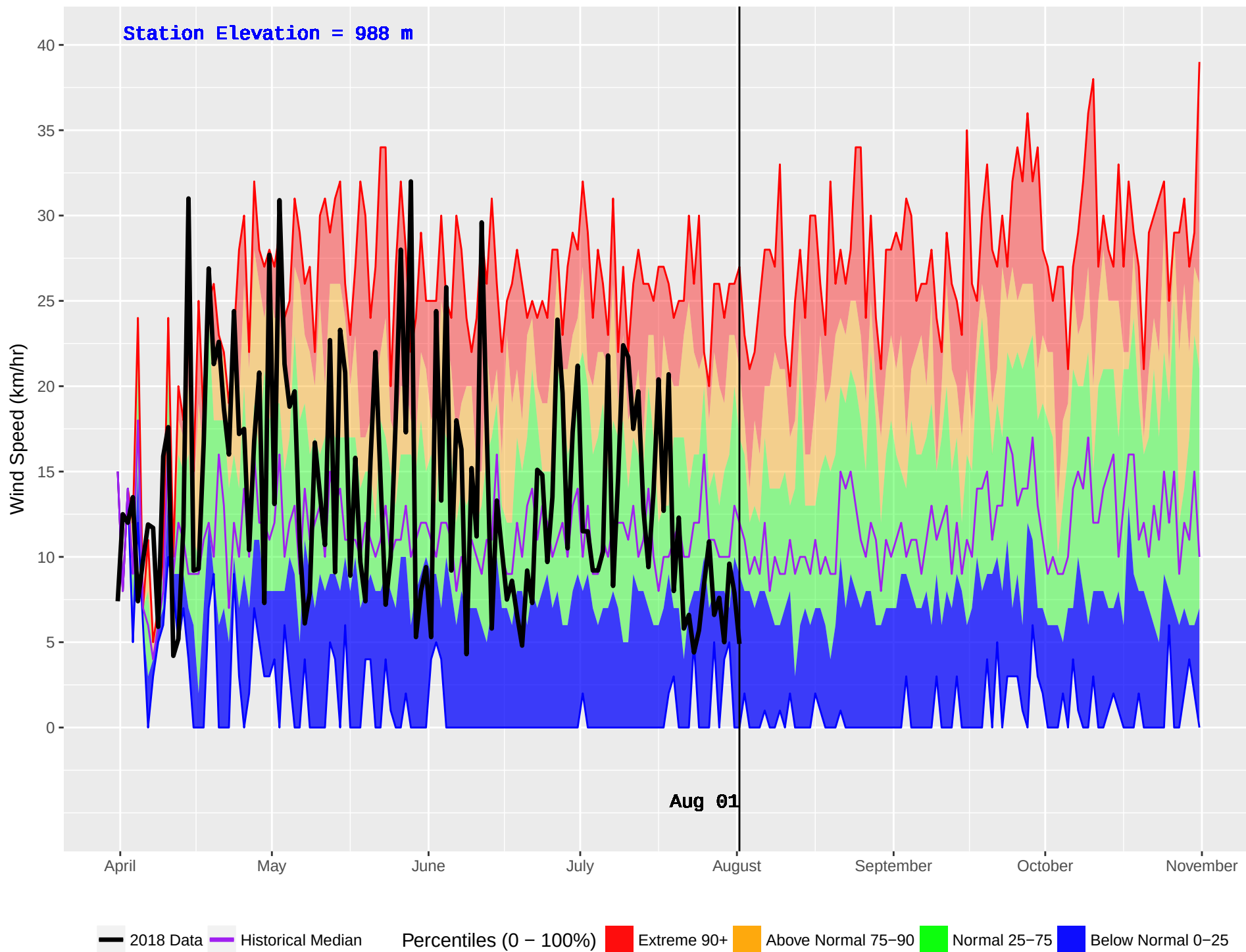
NOEL (437) : Historical (1993–2016) and Current (2018) Daily Wind Speed
