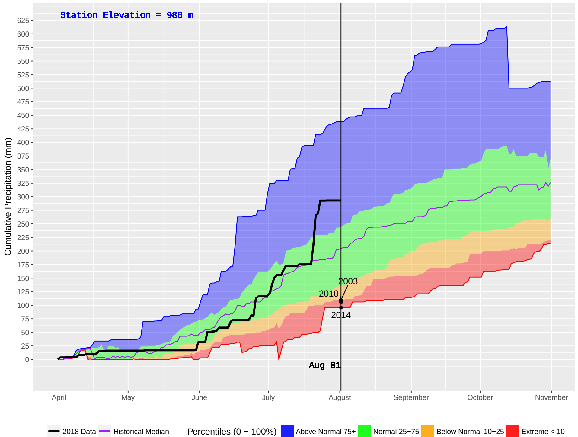
NOEL (437) : Historical (1993–2016) and Current (2018) Daily Cumulative Precipitation
